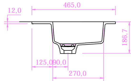
C-C ( 1:10 )
