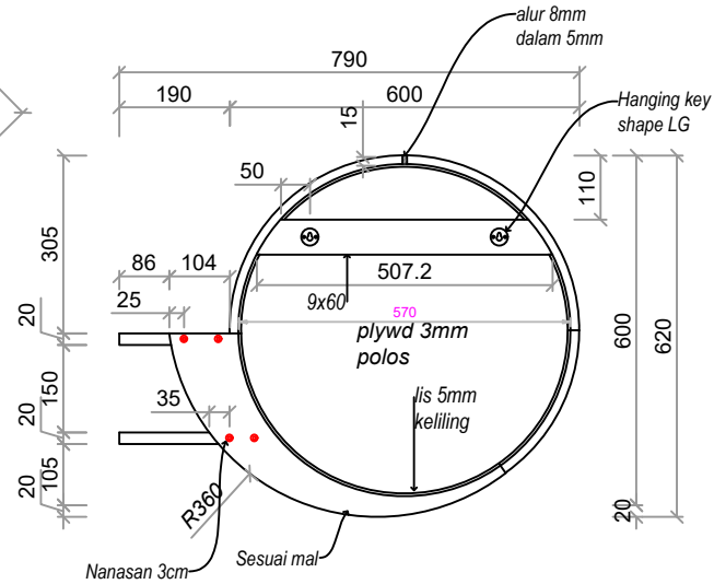
BACK VIEW T. Belakang
