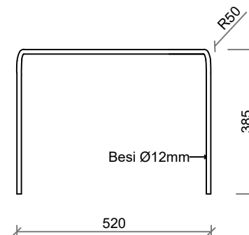
T. SAMPING KAKI BESI SAMPING SCALE 1:10
