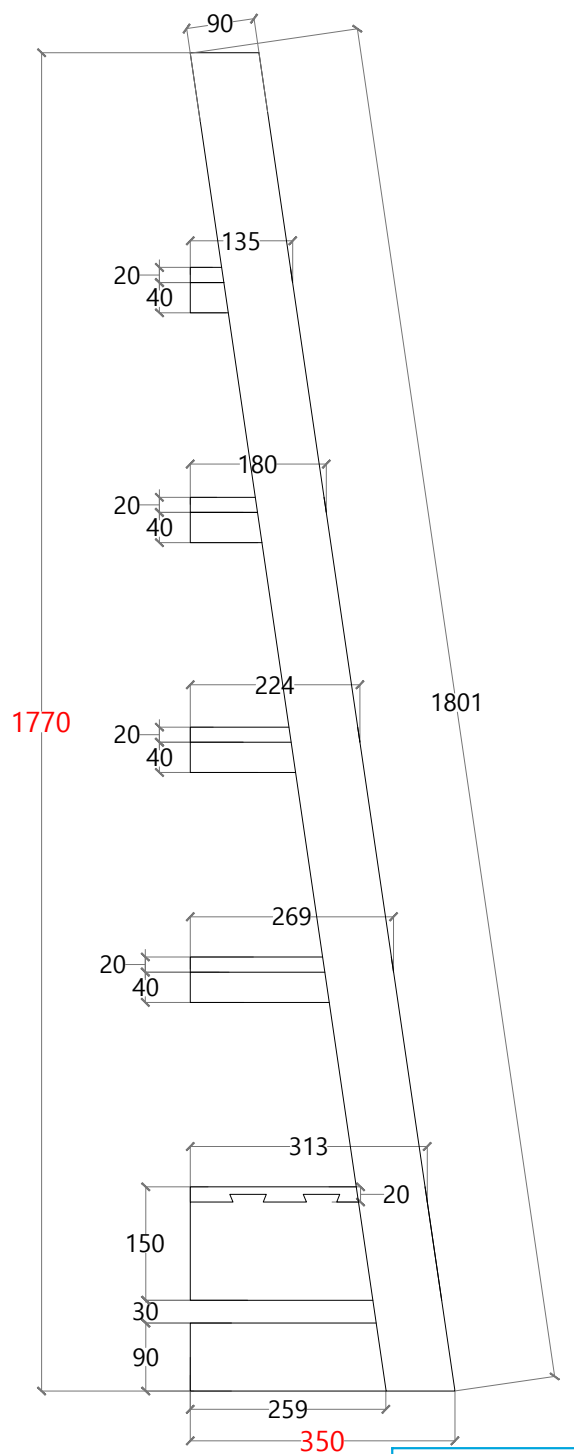
Side VIEW
