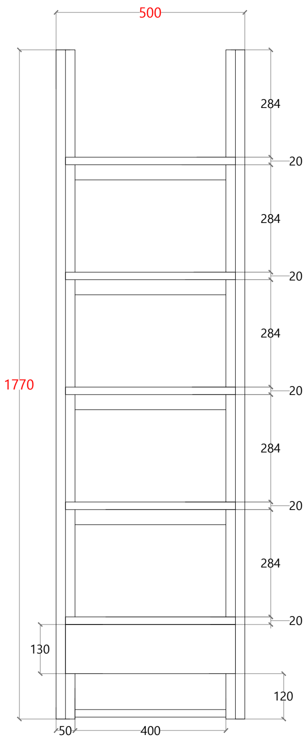
Front VIEW
