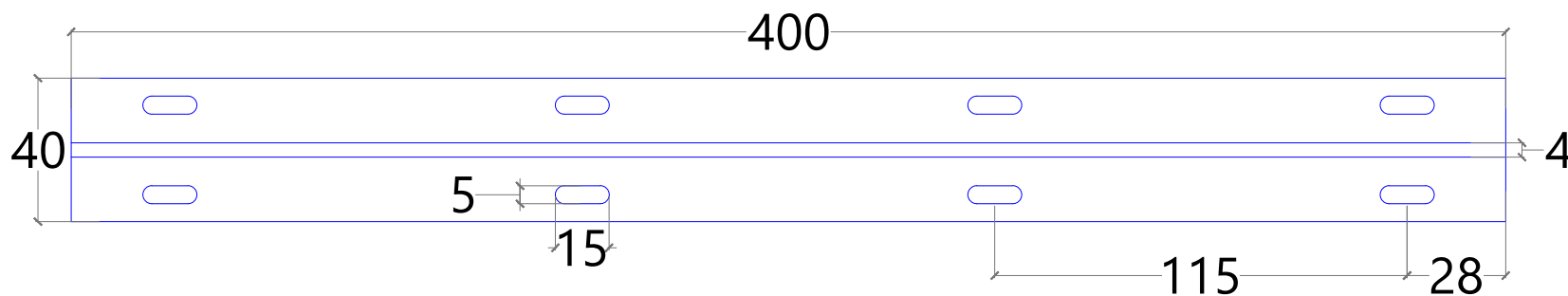
Top VIEW
