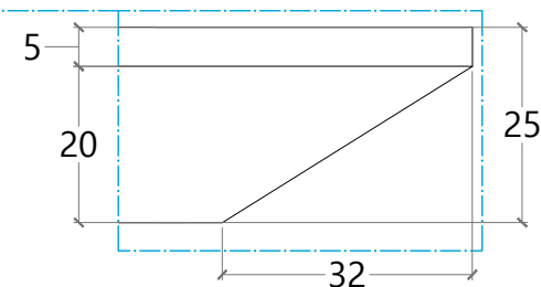
Profile Detail
