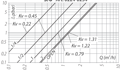
3/8" Art. 0224-0234
