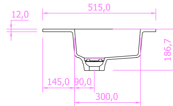
C-C ( 1:10 )
