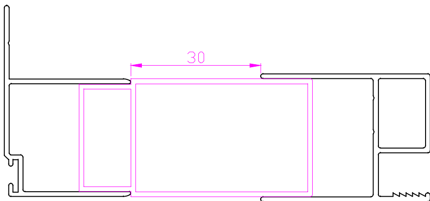
FA801 Wall side
